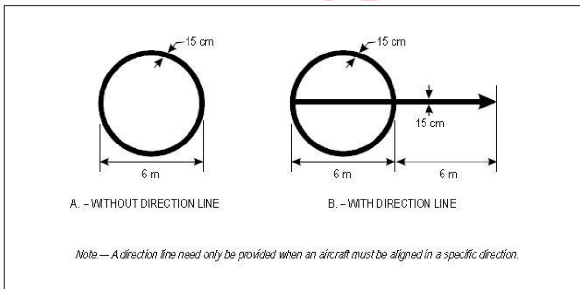
Figure 5-9. VOR aerodrome check-point marking
