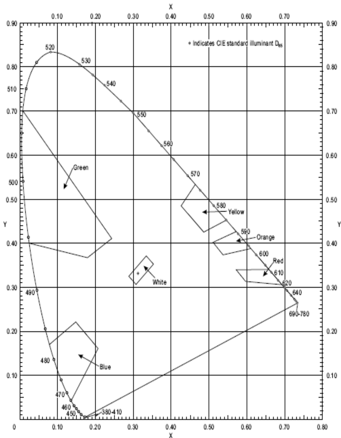
Figure A1-3. Colors of retro-reflective materials for markings, signs and panels
