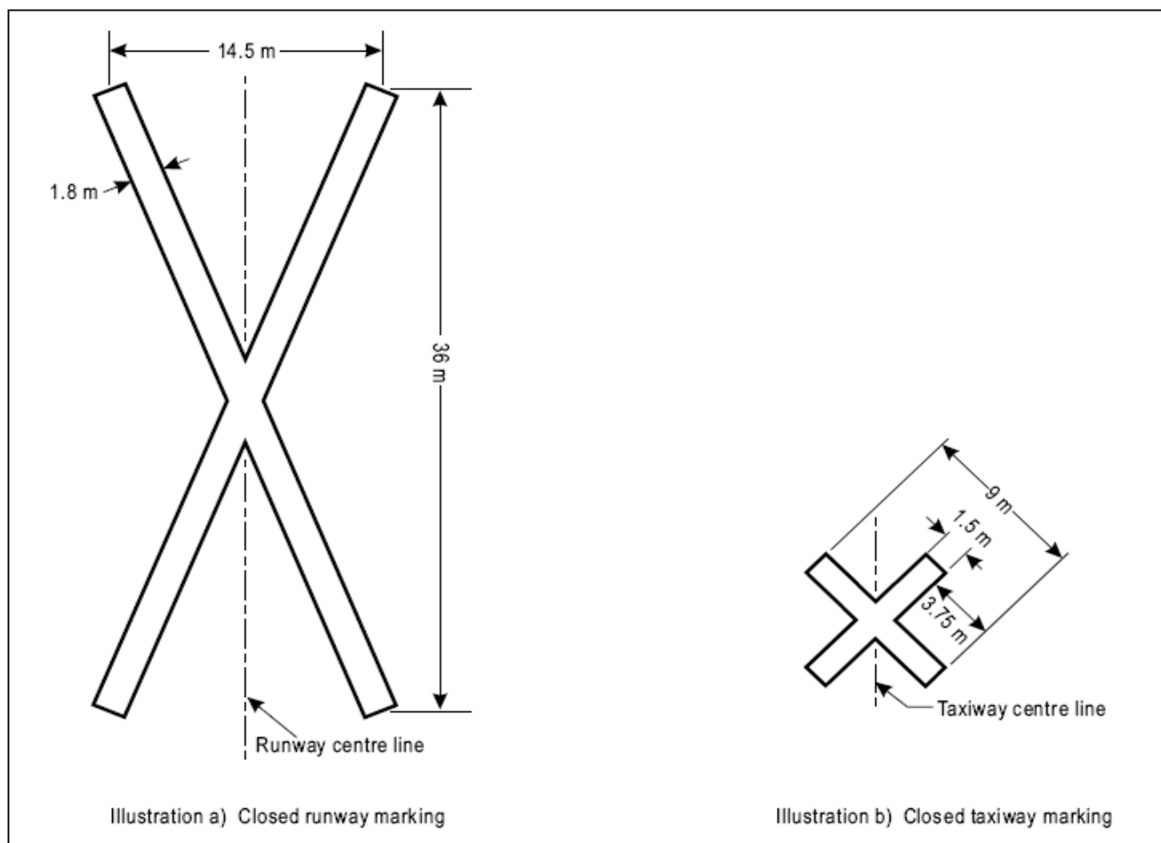
Figure 7-1. Closed runway and taxiway markings
