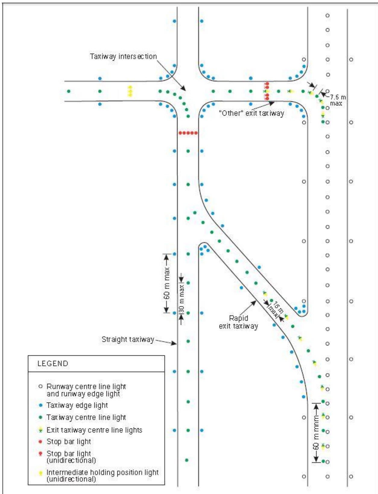
Figure 5-26 Taxiway lighting
