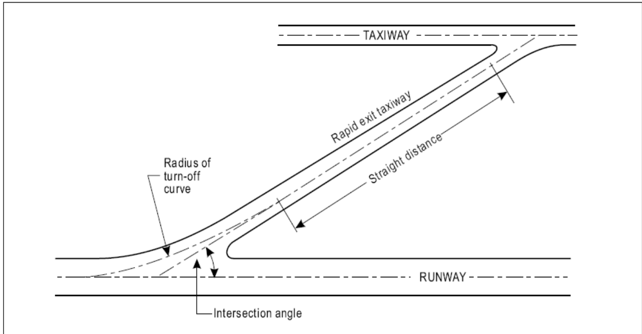
Figure 3-3. Rapid Exit Taxiway
