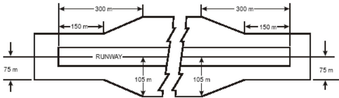
Figure A-3. Graded portion of a strip including a precision approach runway where the code number is 3 or 4
