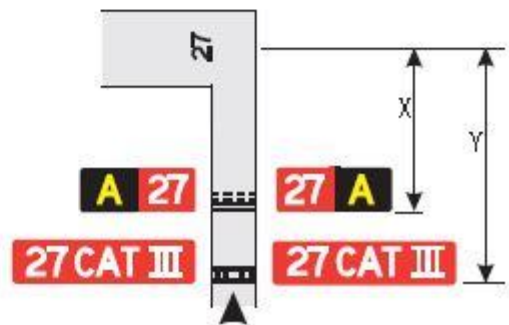
Figure 5-32. Examples of sign positions at taxiway/runway intersections
