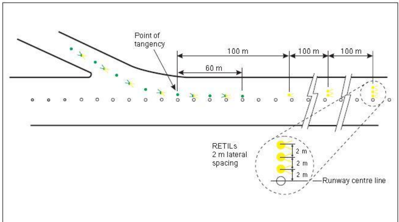
Figure 5.25 Rapid exit taxiway indicator lights (RETILS)
