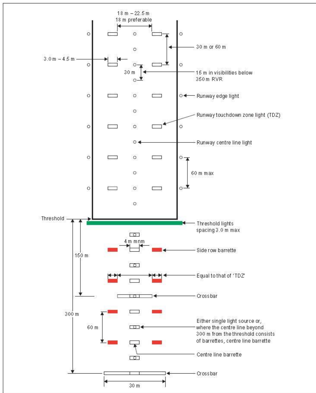
Figure 5-15. Inner 300m approach and runway lighting for precision approach runways categories II and III where the serviceability levels for the lights specified as maintenance objectives in Chapter 10 can be demonstrated
