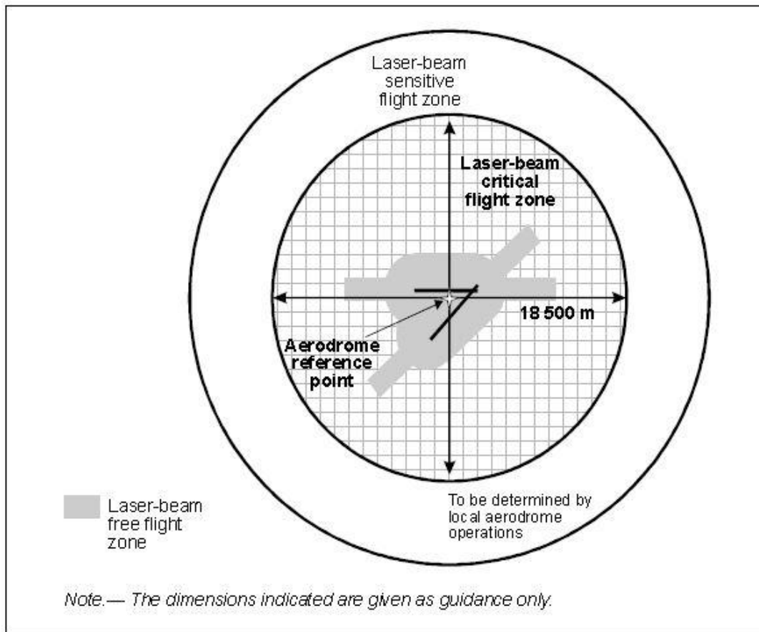
Figure 5-11. Protected flight zone
