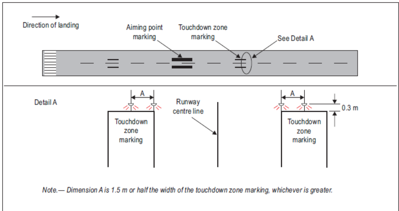
Figure 5-24 Simple touchdown zone lighting
