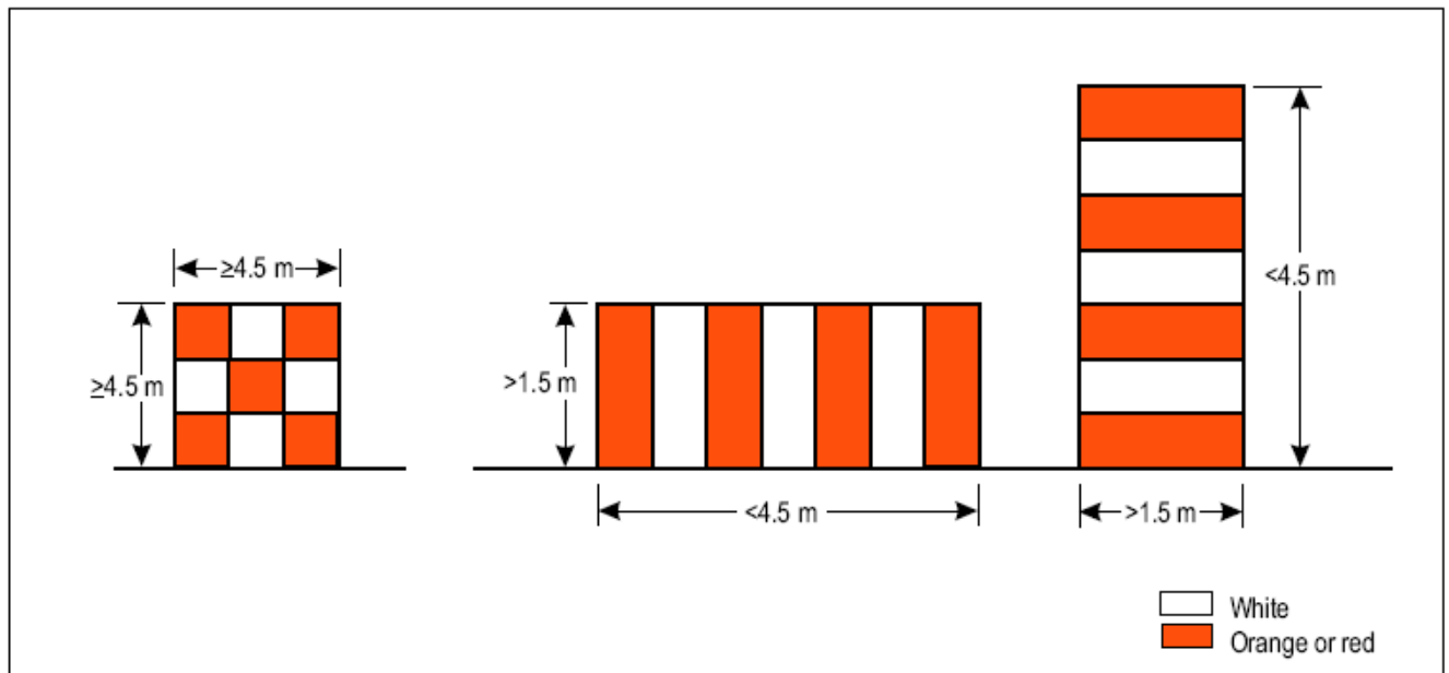
Figure 9.1. Basic marking patterns
