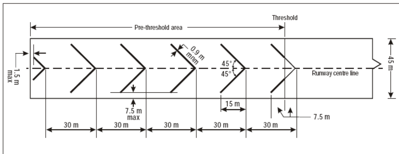
Figure 7-2. Pre-threshold marking
