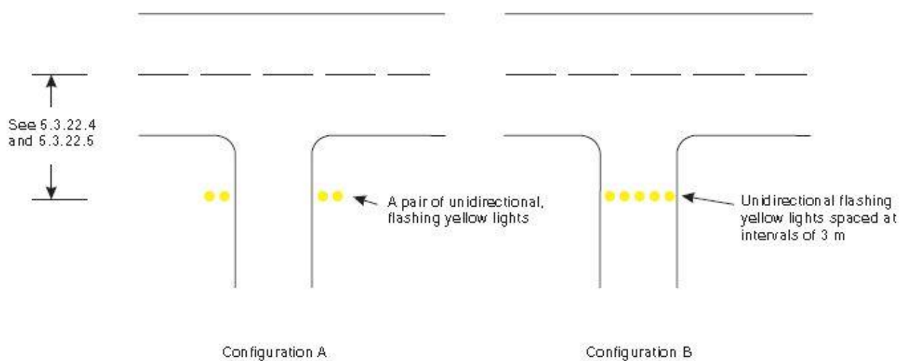
Figure 5.29 Runway guard
