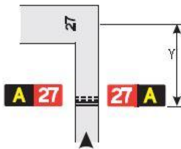
Figure 5-32. Examples of sign positions at taxiway/runway intersections
