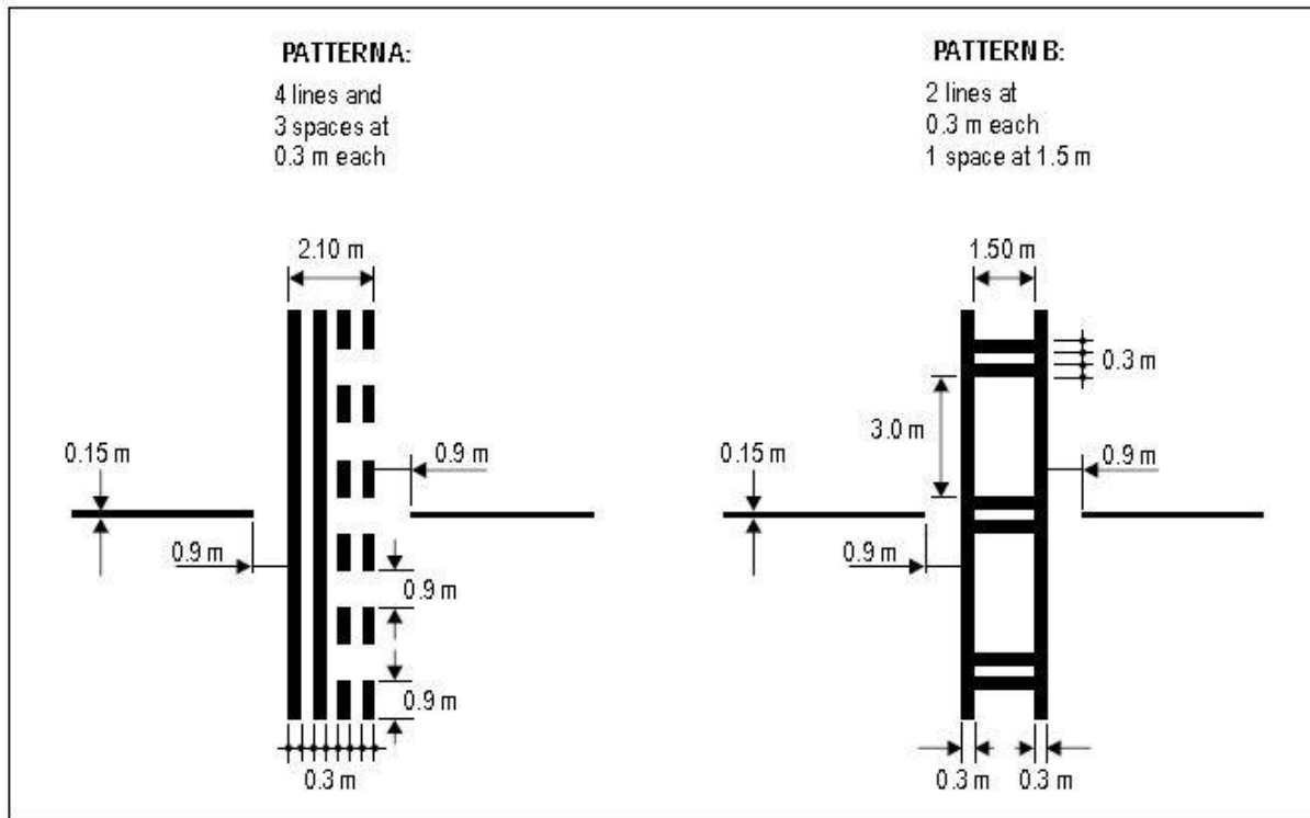
Figure 5-8. Runway-holding position markings
