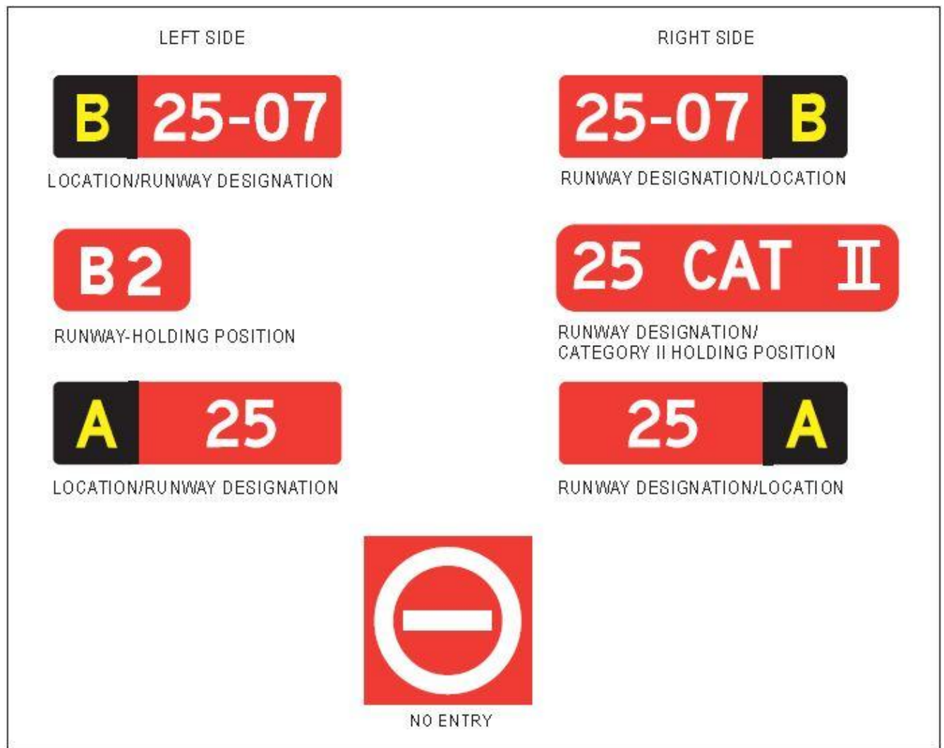
Figure 5.30. Mandatory instruction signs
