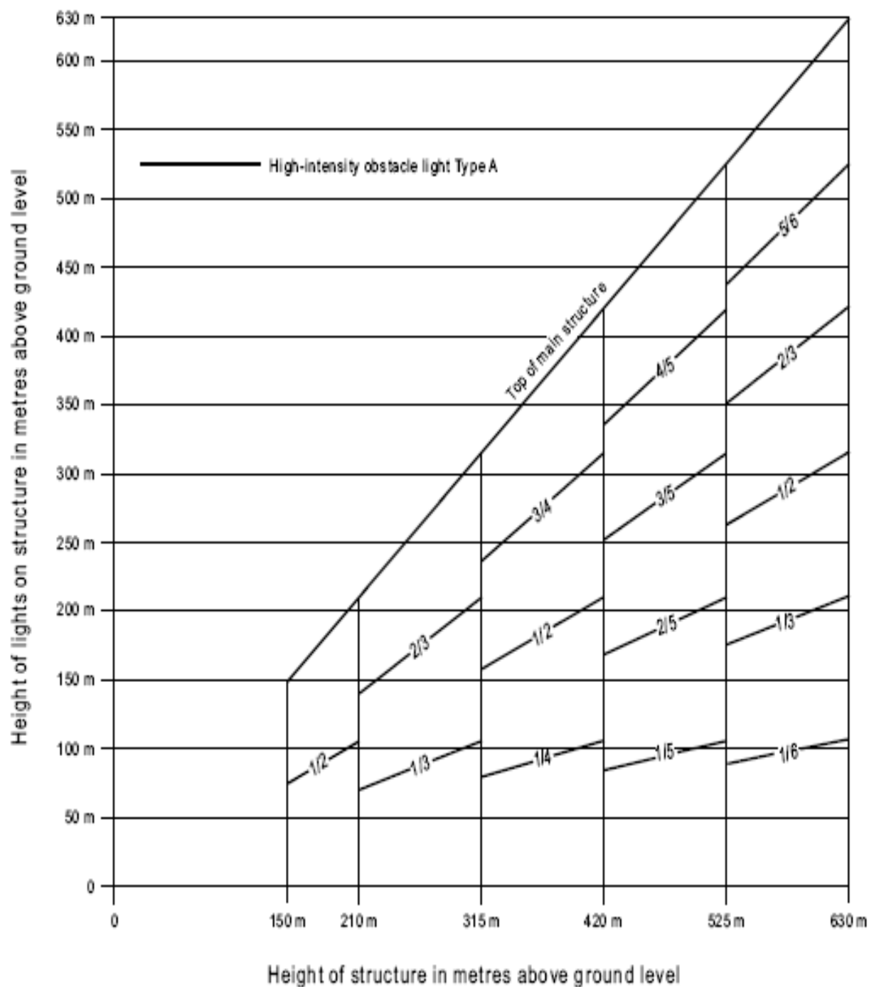
Figure A6-6. High-intensity flashing-white obstacle lighting system, Type A
