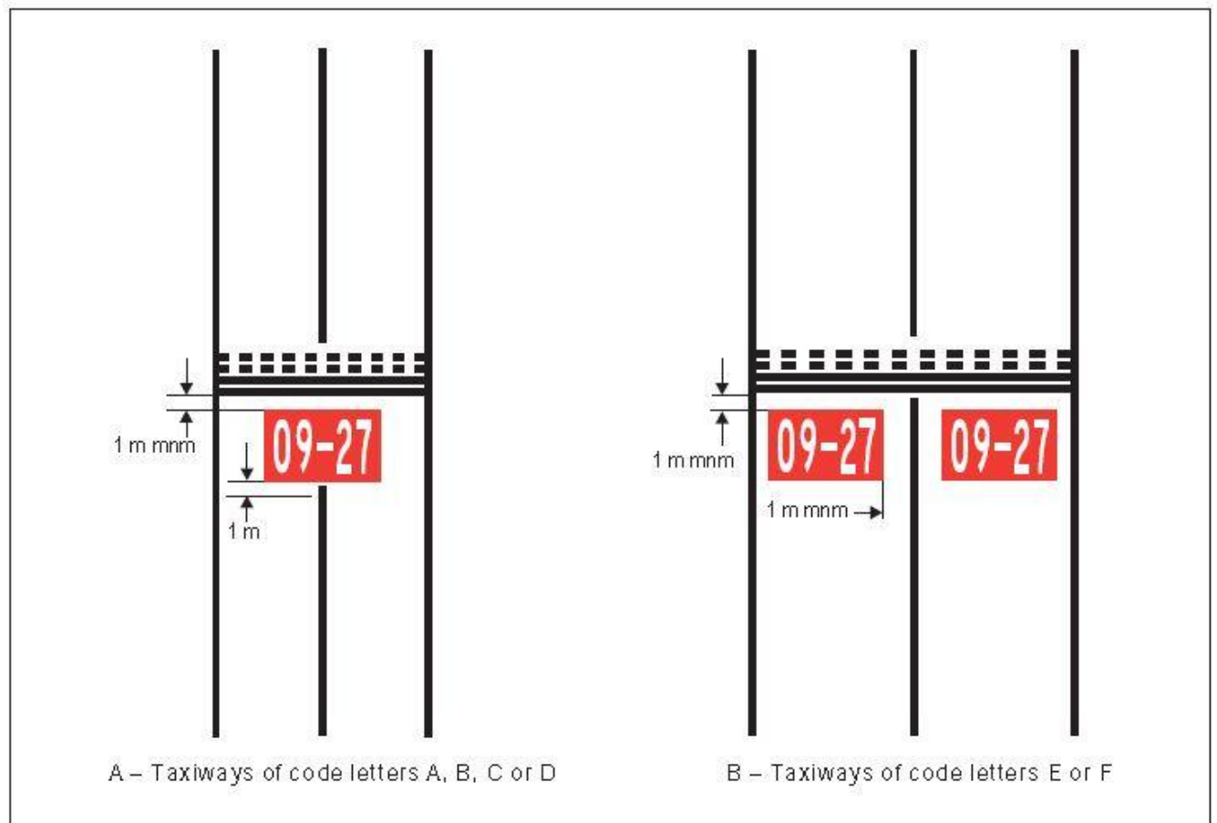
Figure 5-10. Mandatory instruction marking
