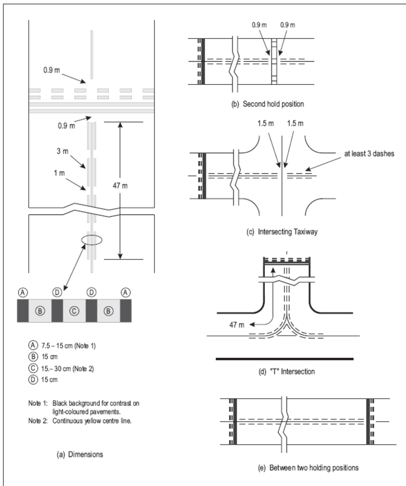
Figure 5-7 Enhanced Taxiway Center Line Marking
