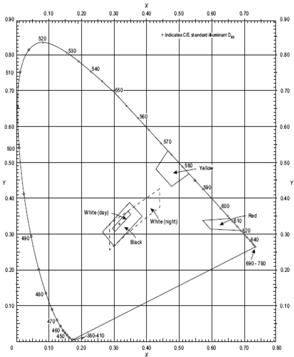
Figure A1-4. Colors of transilluminated (internally illuminated) signs and panels
