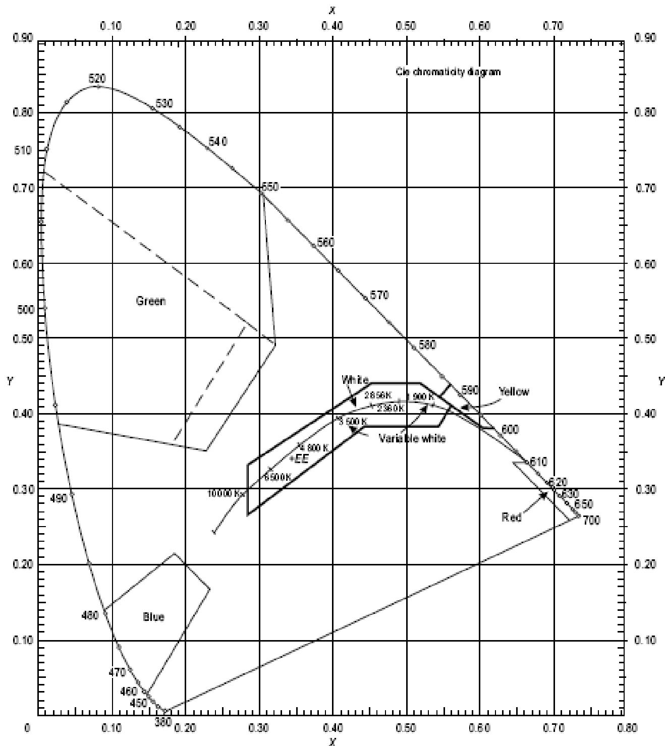
Figure A1-1. Colors for aeronautical ground lights
