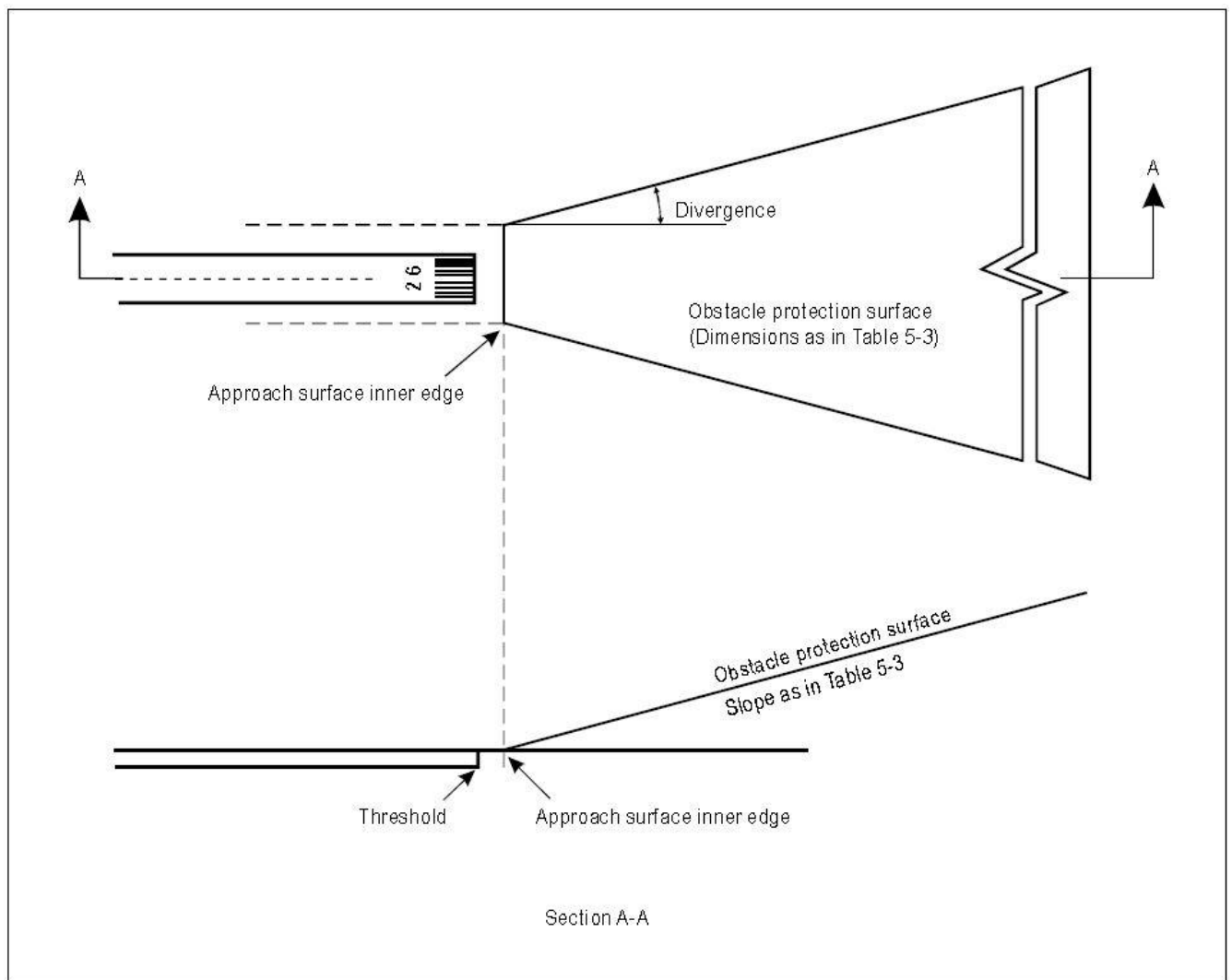
Figure 5-21. Obstacles protection surface for visual approach slope indicator systems
