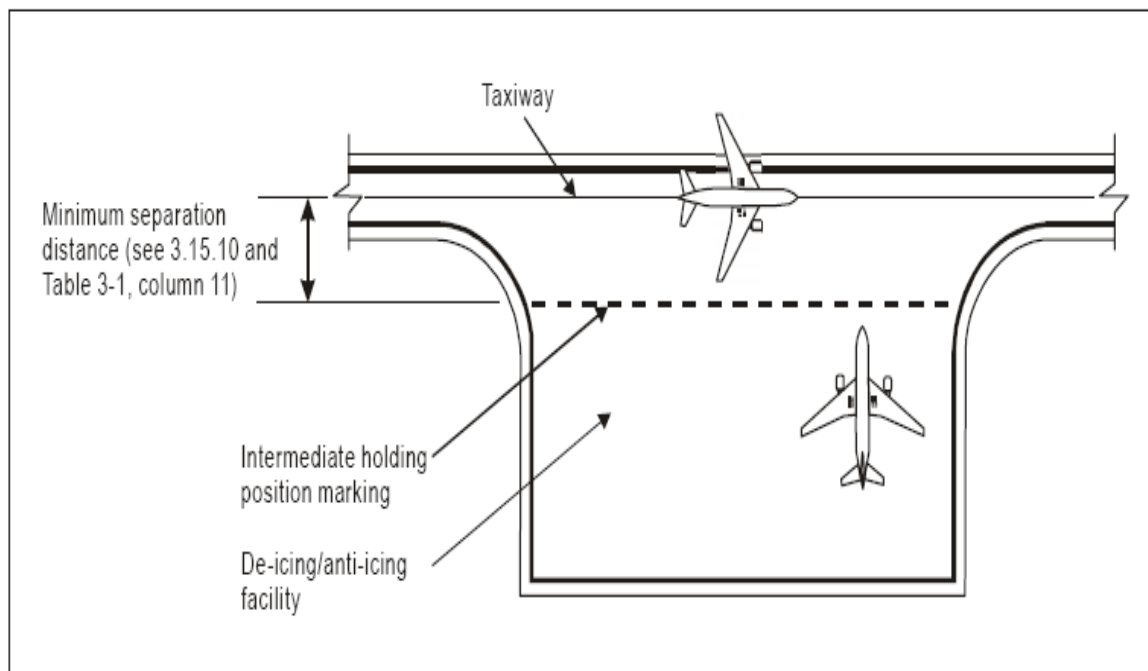
Figure 3-4. Minimum separation distance on a de-icing/anti-icing facility
