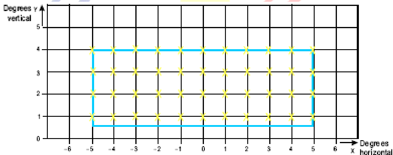
Figure A2.21 Grid points to be used for calculation of average intensity of taxiway center line and stop bar light
