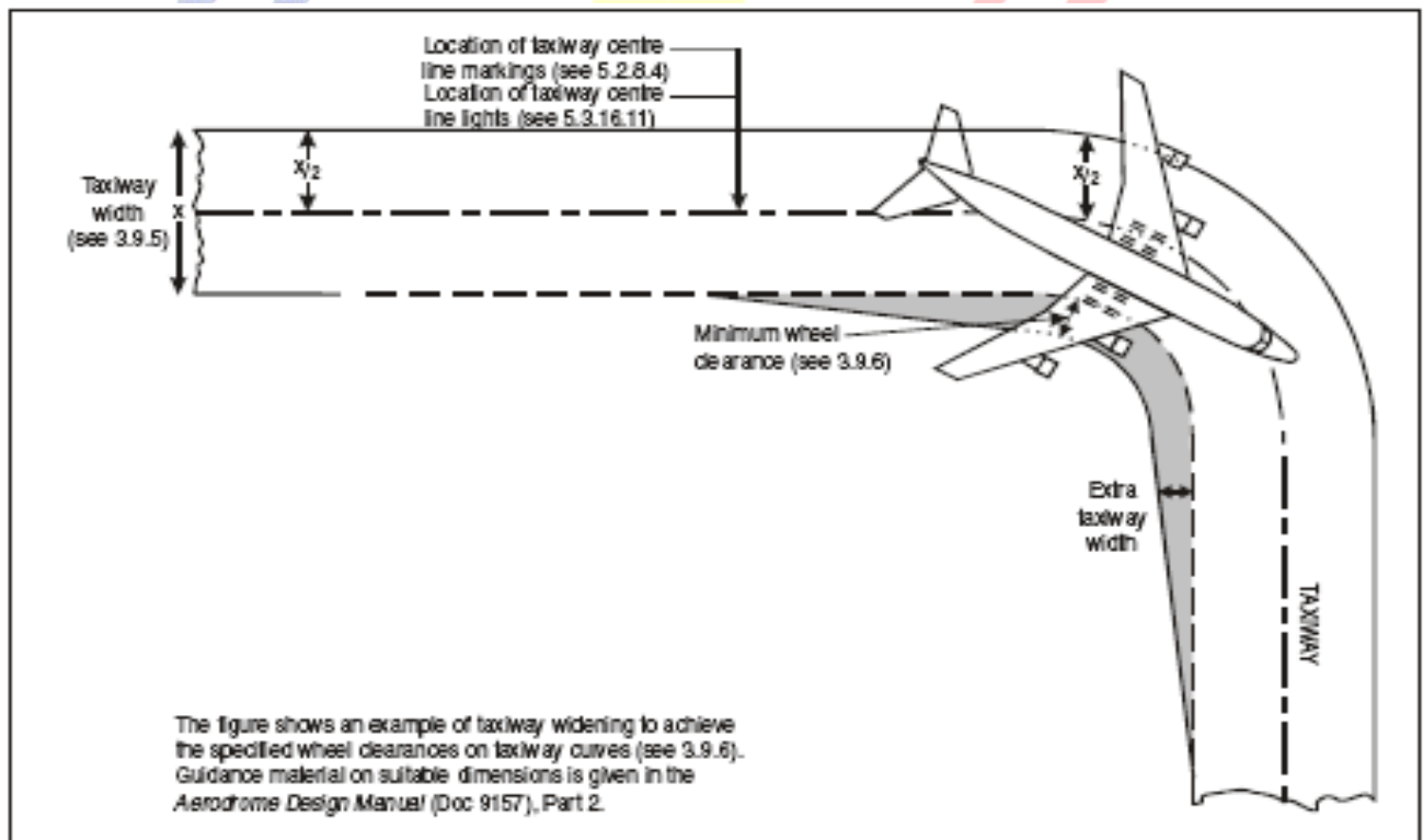
Figure 3-2. Taxiway curve
