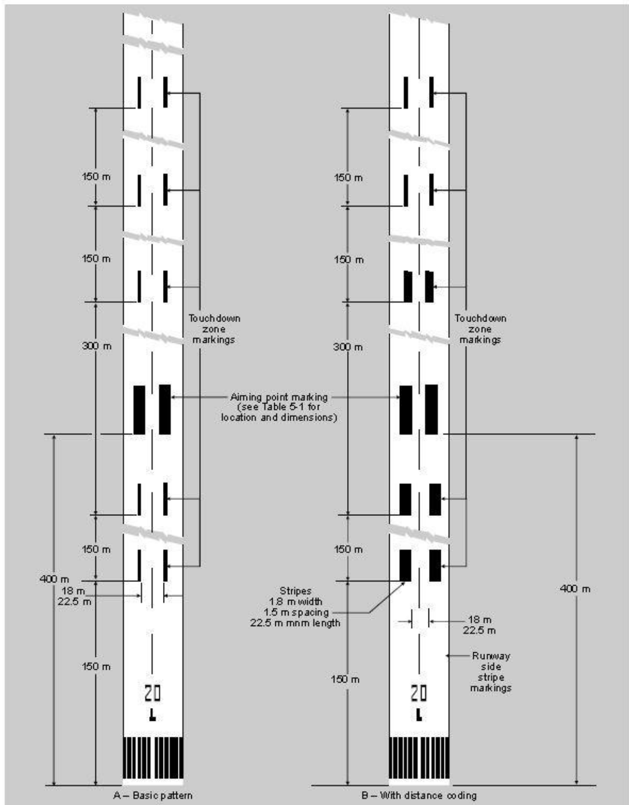
Figure 5-5 Aiming point and touchdown zone markings (illustrated for a runway with a length of 2499 m or more)
