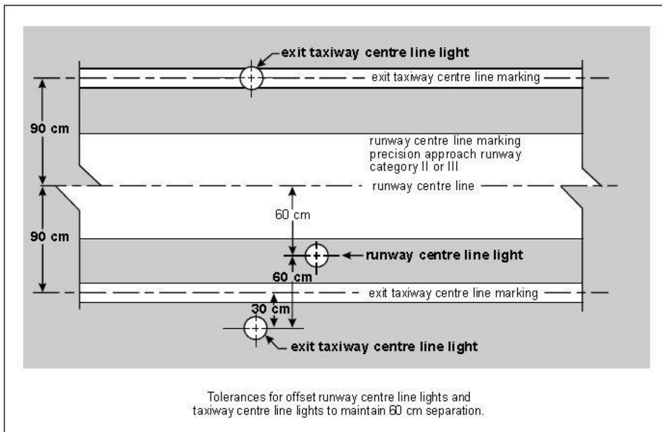
Figure 5-27. Offset runway and taxiway center line lights
